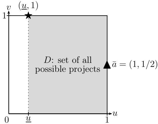
Figure 2: Preliminary intuition, \underline{v} = 0
